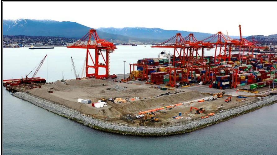
Rip Rap placement
