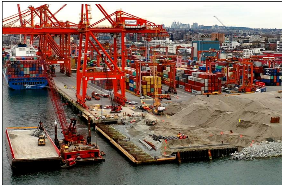
Sheet pile wall and area of precast panel installation
